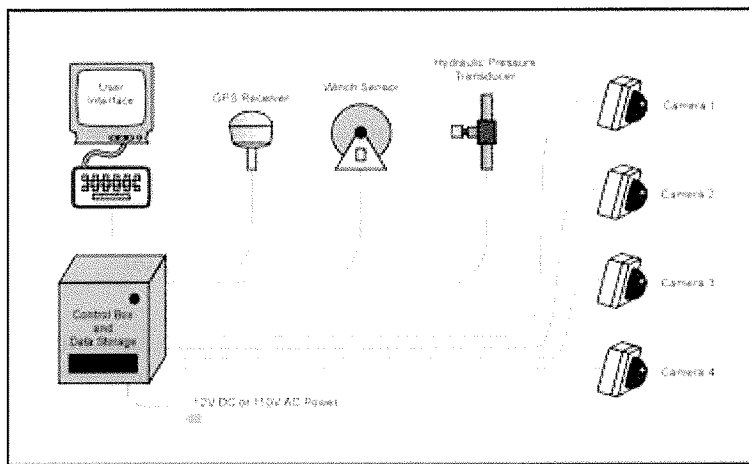
Figure 1 Common Design for Archipelago VBEM System
